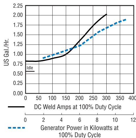
Engine-Driven Welder Fuel Consumption
