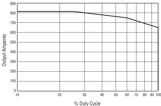
Duty Cycle Chart
